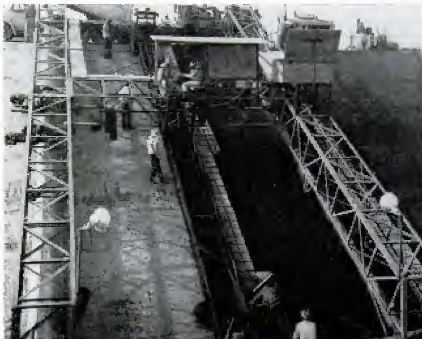
Men with hooks lift wire mesh so that it is embedded in center of asphalt
